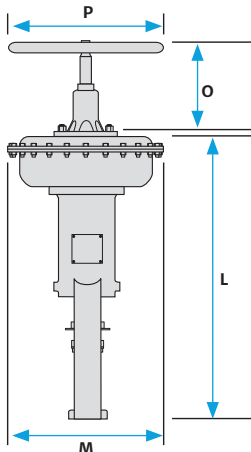
Direct Acting (Spring-to-Open)
